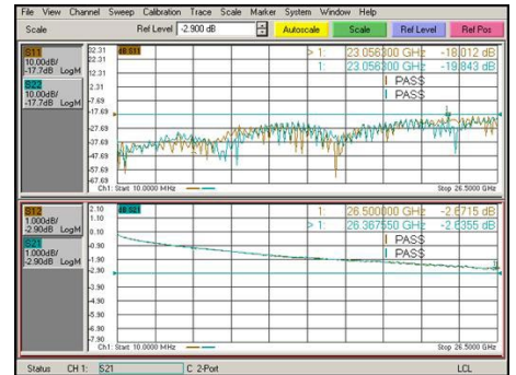
Test: SMA Male to SMA Male, 24 inches, DC - 26.5 GHz
