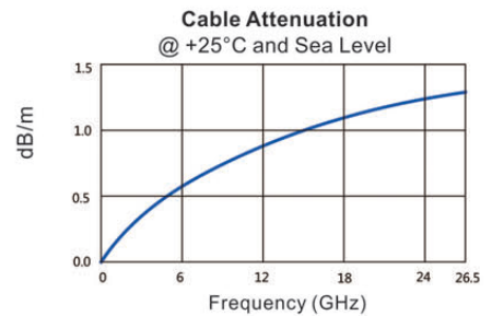
Test: SMA Male to SMA Male, 24 inches, DC - 26.5 GHz
